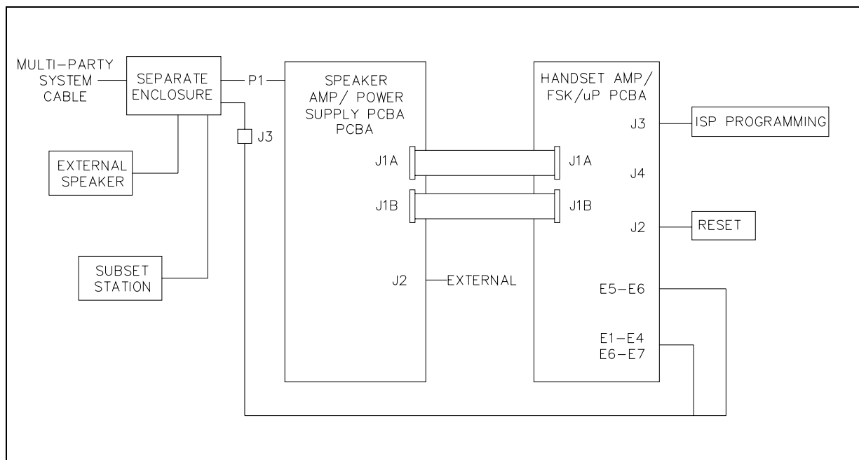
Figure 3. Remote Subset Amplifier Block Diagram
