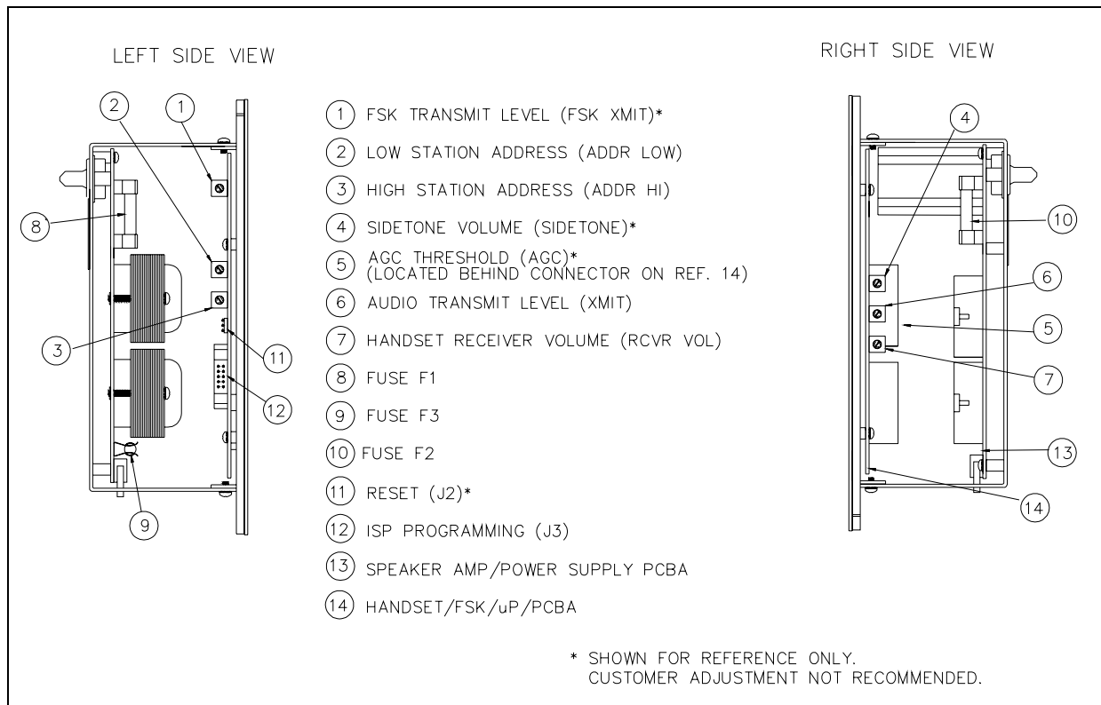
Figure 2. Remote Subset Amplifier Outline Detail
