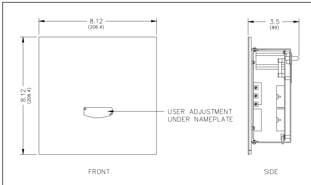
Figure 1. Remote Subset Amplifier - Front Outline and Side View
